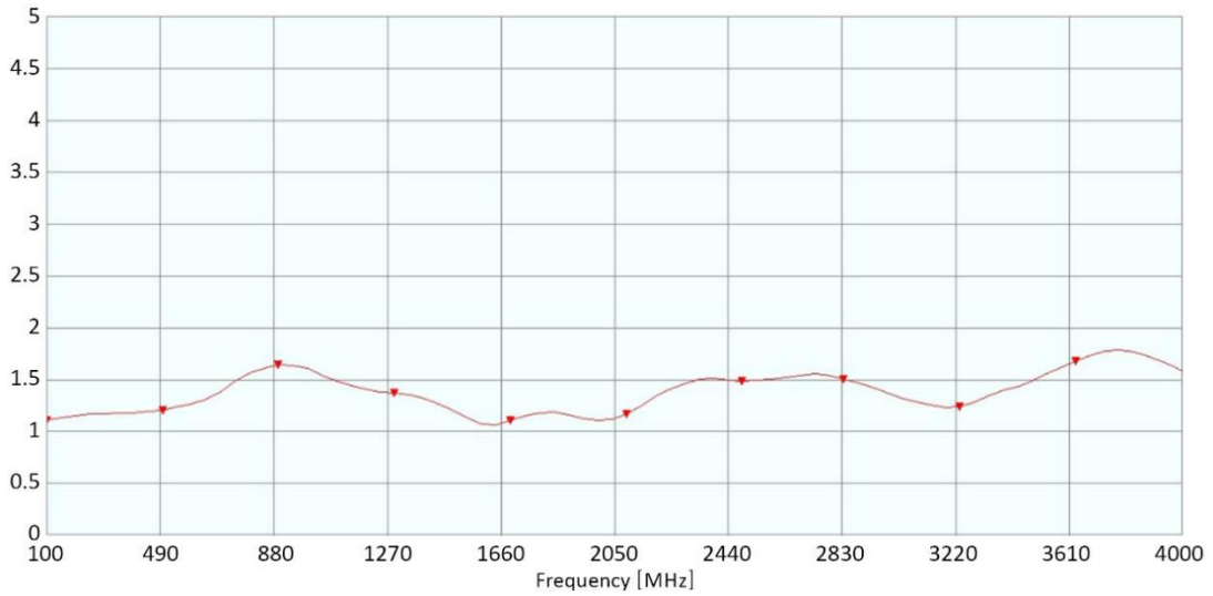
Figure 9: Typical VSWR 875-12 & 875-20
