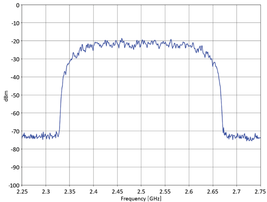
Figure 31: 16QAM 250 MS/s
